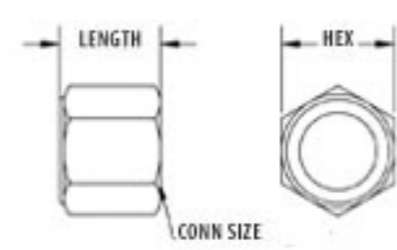
Female - 1/8" - 1/2"
